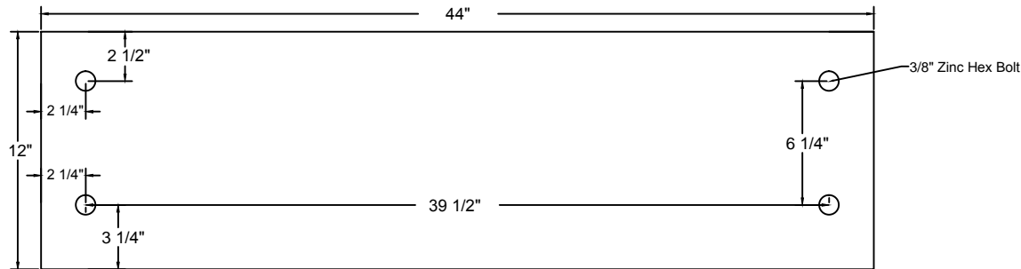
Stringer View
